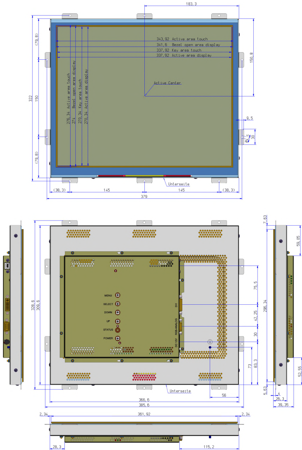
Figure 1: Mechanical Outlines
