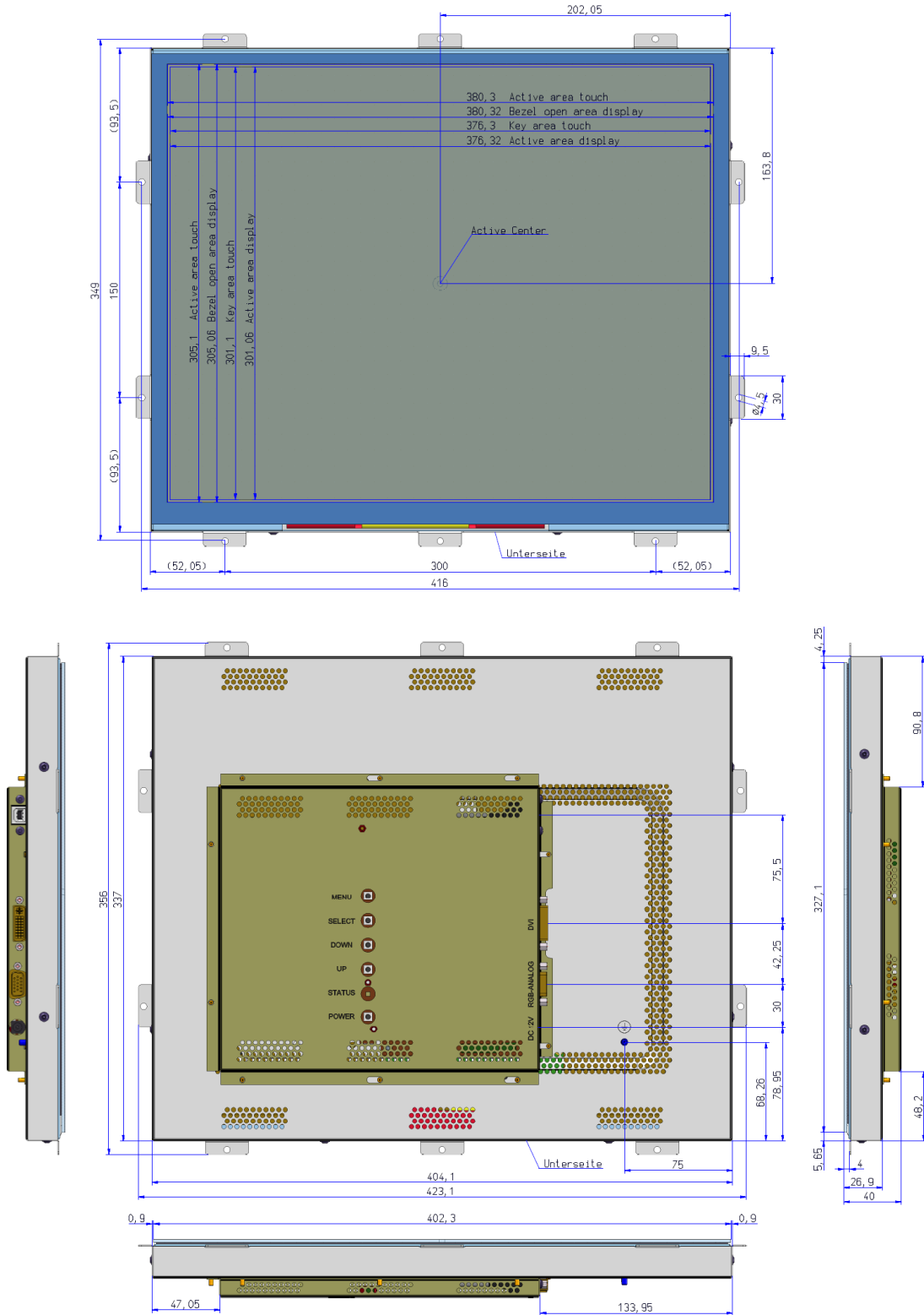
Figure 1: Mechanical Outlines
