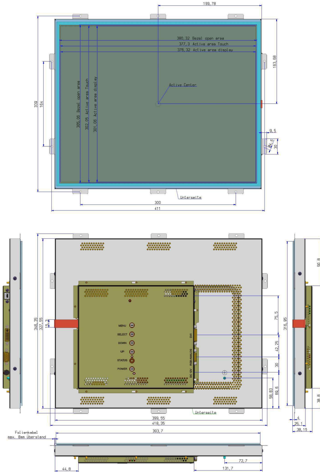
Figure 1: Mechanical Outlines
